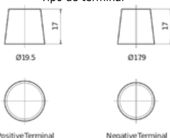
Positive Terminal
